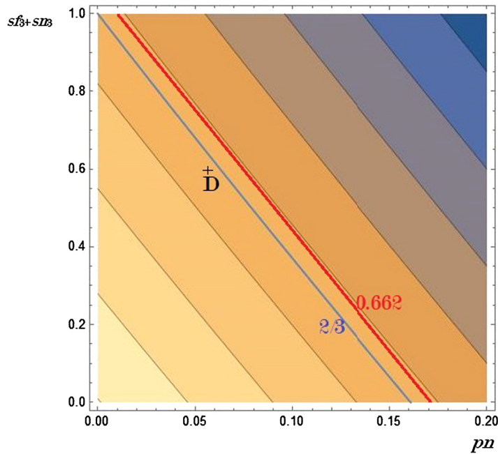
Fig. A.1. Decomposing the return to social information at position 4: Level curves for \pi(sf_4) . Rate of non-compliance pn (on x-axis) vs. frequency of choice of social information sf_3 + sn_3 at position 3 (on y-axis), with the empirical average denoted by D . The maximum value \pi(sf_4) = q^3 + 3q^2(1-q) = 20/27 \approx 0.741 at the origin. The level curve representing the empirical average of \pi(sf_4) = 0.662 is in red, and the level curve representing the return to private information q = \frac{2}{3} is in blue.
